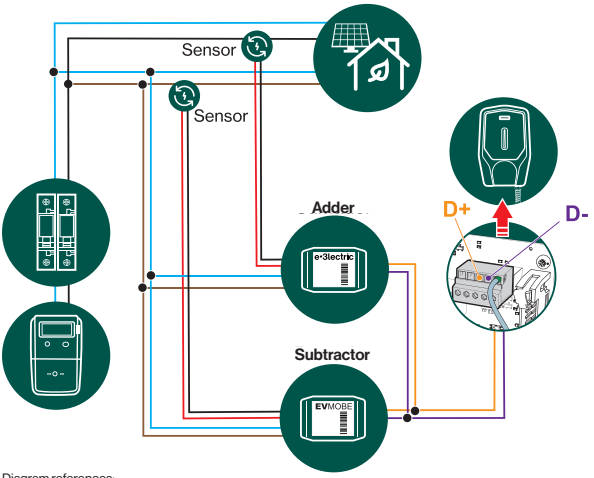
Diagram references: 97111 and 97121. Single phase
