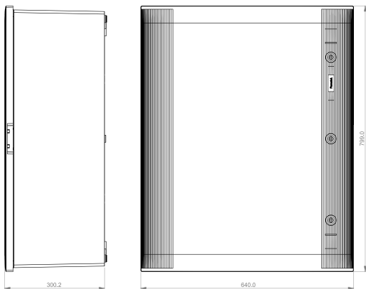
Armario / Enclosure - Ref. Item 49168-T-3P / 49168-3P
