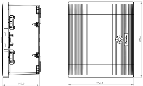
Armario / Enclosure - Ref. Item 49123
