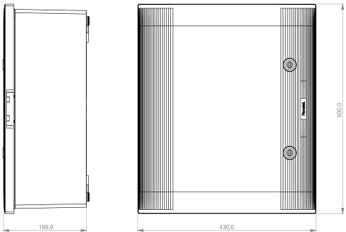
Armario / Enclosure - Ref. Item 49146-T / 49146
