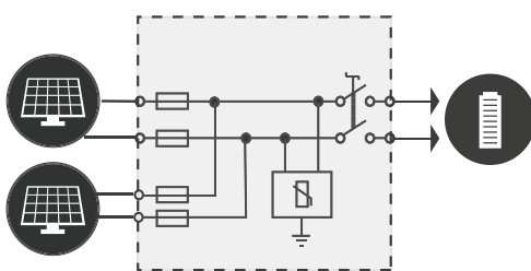
*Esquema Ref. E3SBDC12-FVC2SE *Ref.E3SBDC12-FVC2SE diagram
