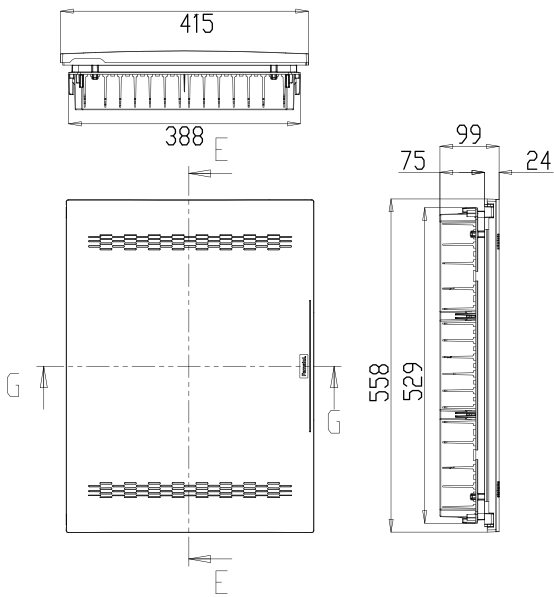
Armario / Enclosure - Ref. Item 32054-F
