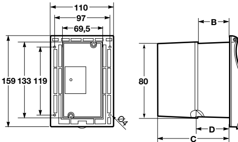
Clavija empotrable basculante para caravana IP44 / Fush mounting plug for caravan IP44
