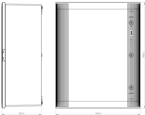
Armario / Enclosure - Ref. Item 49186
