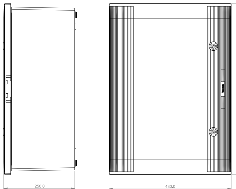
Armario / Enclosure - Ref. Item 49146-T / 49146
