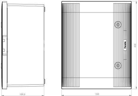
Armario / Enclosure - Ref. Item 49134-T / 49134
