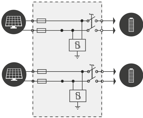
*Esquema Ref. E3SBDC26-FVC2SS *Ref.E3SBDC26-FVC1SP diagram
