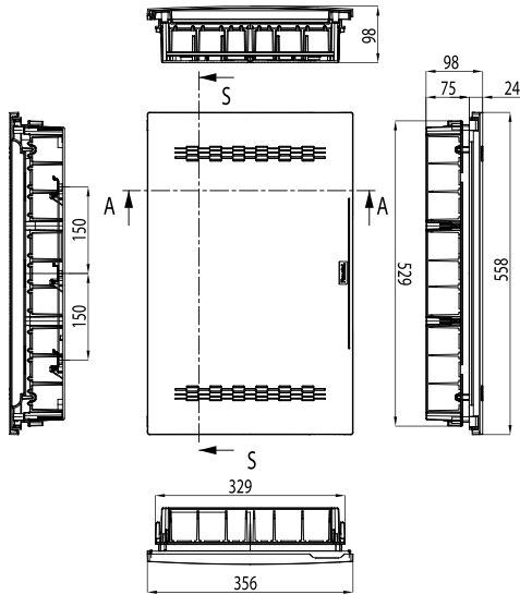
Armario / Enclosure - Ref. Item 32054-F
