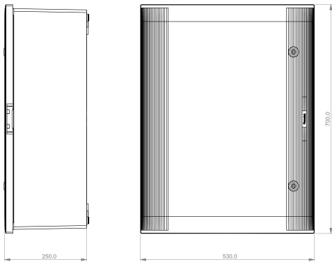
Armario / Enclosure - Ref. Item 49168-T / 49168
