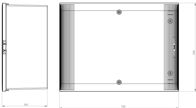
Armario / Enclosure - Ref. Item 49186
