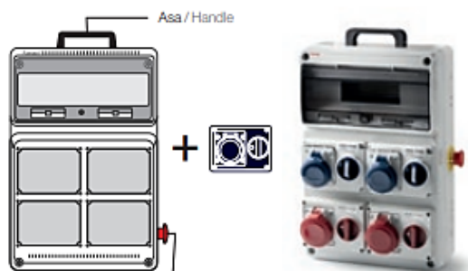
Asa / Handle Seta de emergencia / Emergency push button Ref. / Item 3970 Ref. / Item 6901
